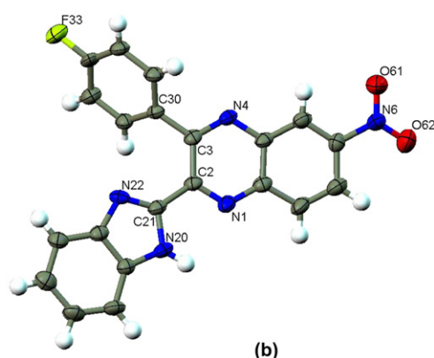
Fig. 3. ORTEP drawing of 7a (a) and 8a (b) molecules. Displacement ellipsoids are drawn at the 30% probability level. H atoms are represented by circles of arbitrary radii. The solvent molecule in (a) was omitted for clarity.
