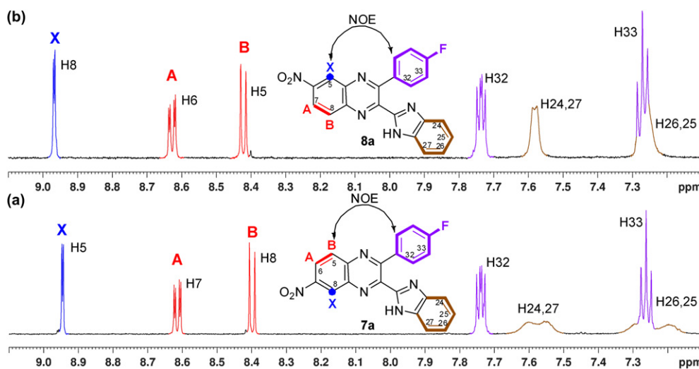
Fig. 2. Fragments of ^1\text{H} NMR spectra (DMSO, 303 K) of 7a (a) and 8a (b). Observed NOE's are shown schematically by arrows.
