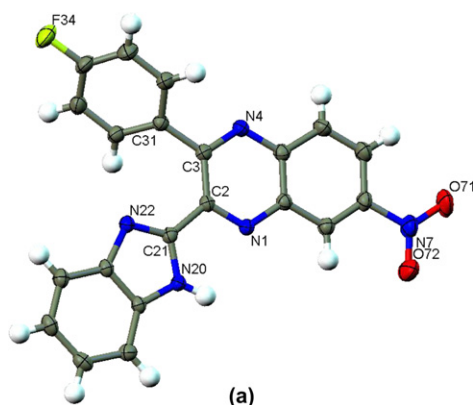
Fig. 3. ORTEP drawing of 7a (a) and 8a (b) molecules. Displacement ellipsoids are drawn at the 30% probability level. H atoms are represented by circles of arbitrary radii. The solvent molecule in (a) was omitted for clarity.
