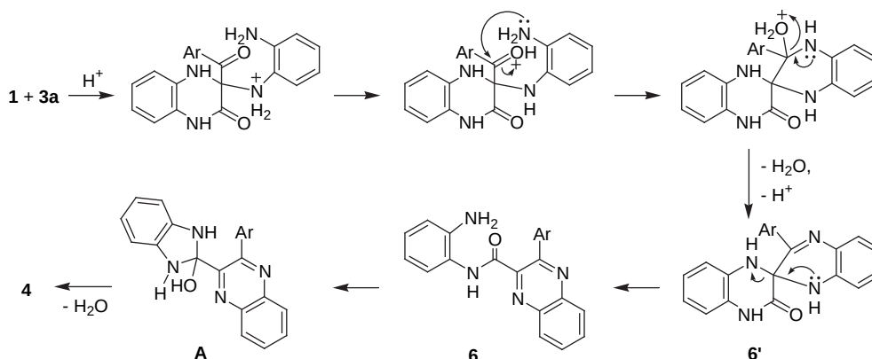
Scheme 2. A probable mechanism of the rearrangement.
