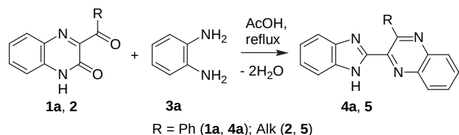
Scheme 1. A new acid-catalyzed rearrangement, proceeding in the 'quinoxalinone—1,2-phenylenediamine' system.
