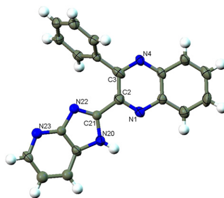
Fig. 4. ORTEP plot of compound 10a . Displacement ellipsoids are drawn at the 30% probability level. The solvent water molecules were omitted for clarity.
