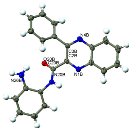
Fig. 1. ORTEP drawing one of the two independent 6a molecules. Displacement ellipsoids are drawn at the 30% probability level and H atoms are shown as small spheres of arbitrary radii.
